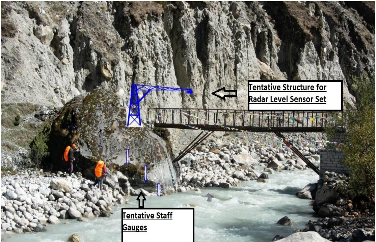
Fig. Tentative site for Installation and Commissioning of Radar Level Sensor Set at Pangboche along with tentative staff gauge.
