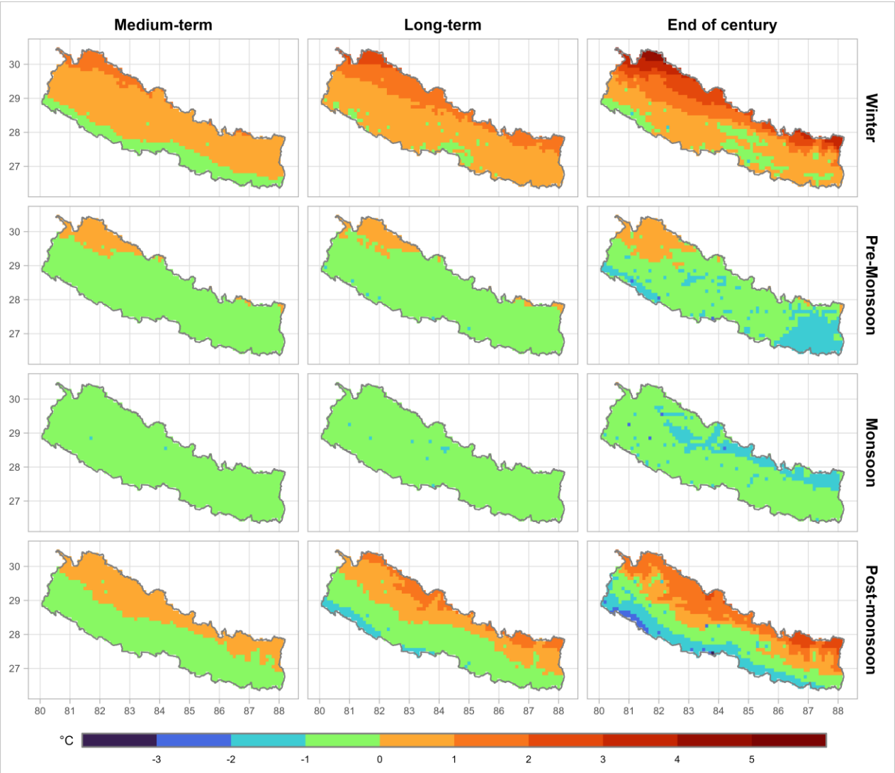
Figure 8.15: Spatiotemporal variation of projected change in seasonal diurnal temperature range (°C) during medium-term, long-term and end of century compared to the baseline period (1981–2010) for SSP5-8.5 scenario. Results are an ensemble average of selected four models
