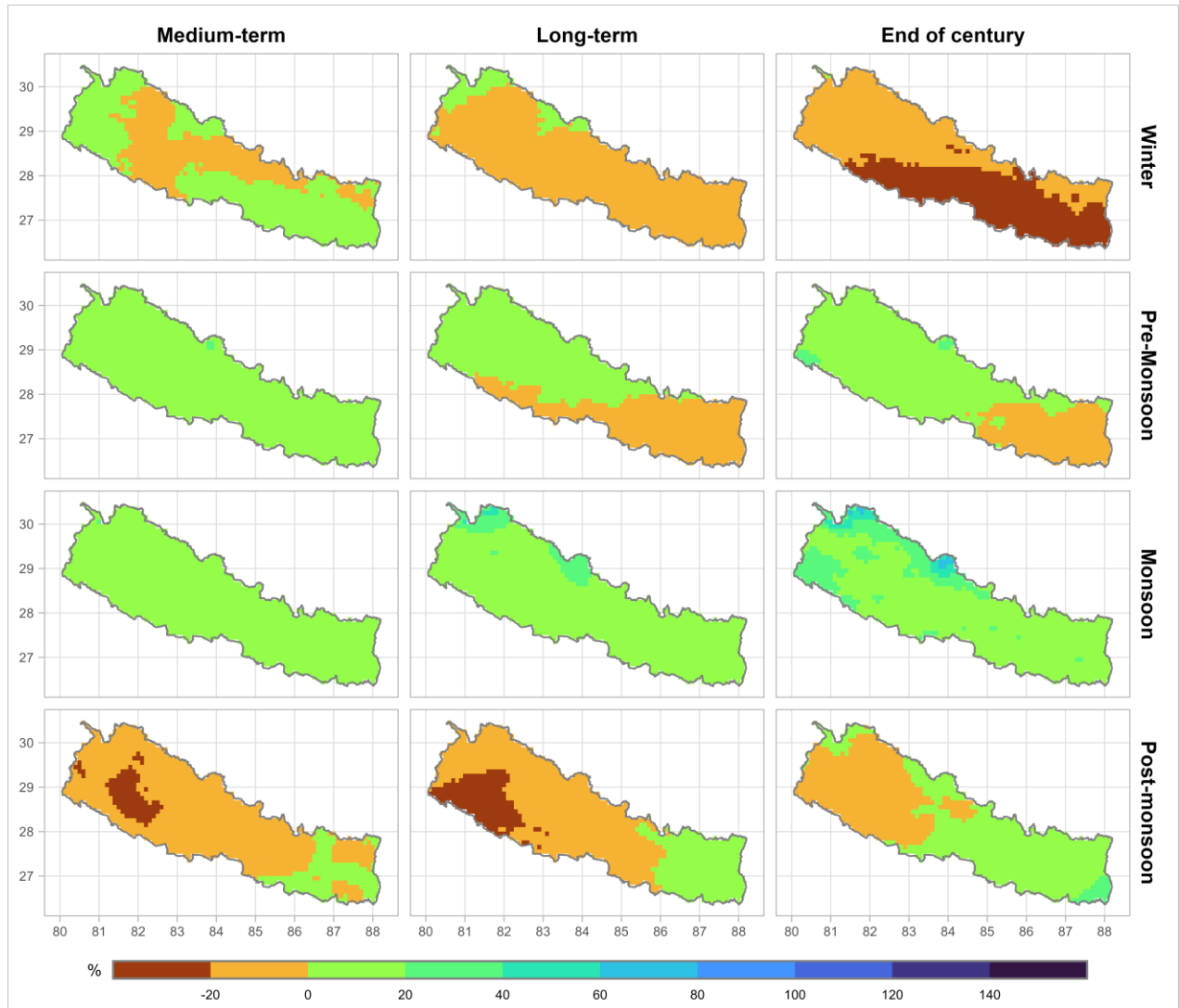
Figure 8.6: Spatiotemporal variation of projected change in seasonal precipitation (%) during medium-term, long-term and end of century compared to the baseline period (1981–2010) for SSP2-4.5 scenario. Results are an ensemble average of selected four models.
