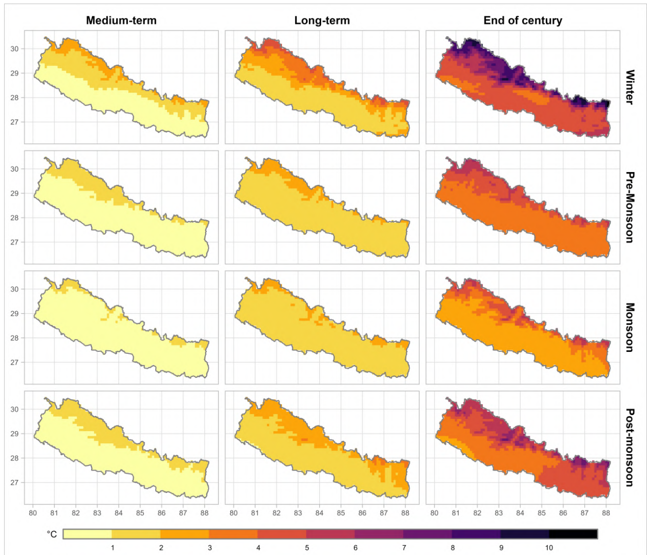
Figure 8.11: Spatiotemporal variation of projected change in seasonal maximum temperature (°C) during medium-term, long-term and end of century compared to the baseline period (1981–2010) for SSP5-8.5 scenario. Results are an ensemble average of selected four models.
