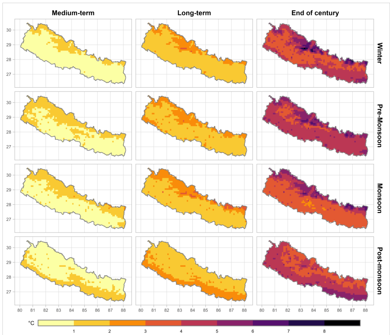
Figure 8.13: Spatiotemporal variation of projected change in seasonal minimum temperature (°C) during medium-term, long-term and end of century compared to the baseline period (1981–2010) for SSP5-8.5 scenario. Results are an ensemble average of selected four models.
