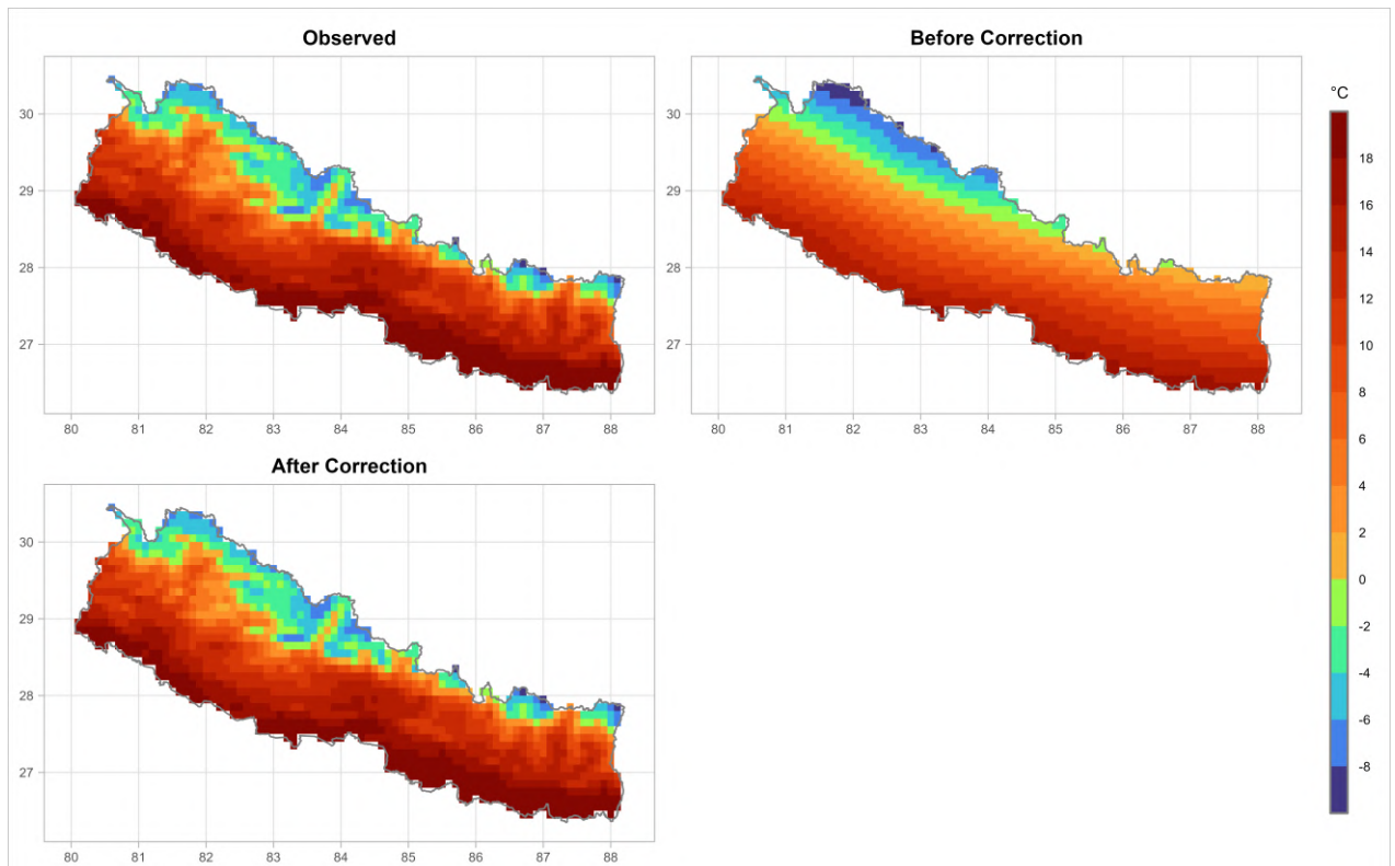
Figure 11: Comparison of observed and simulated average annual maximum temperature before and after downscaling. The "before" and "after" correction panels display the ensemble mean values derived from the selected GCMs.
