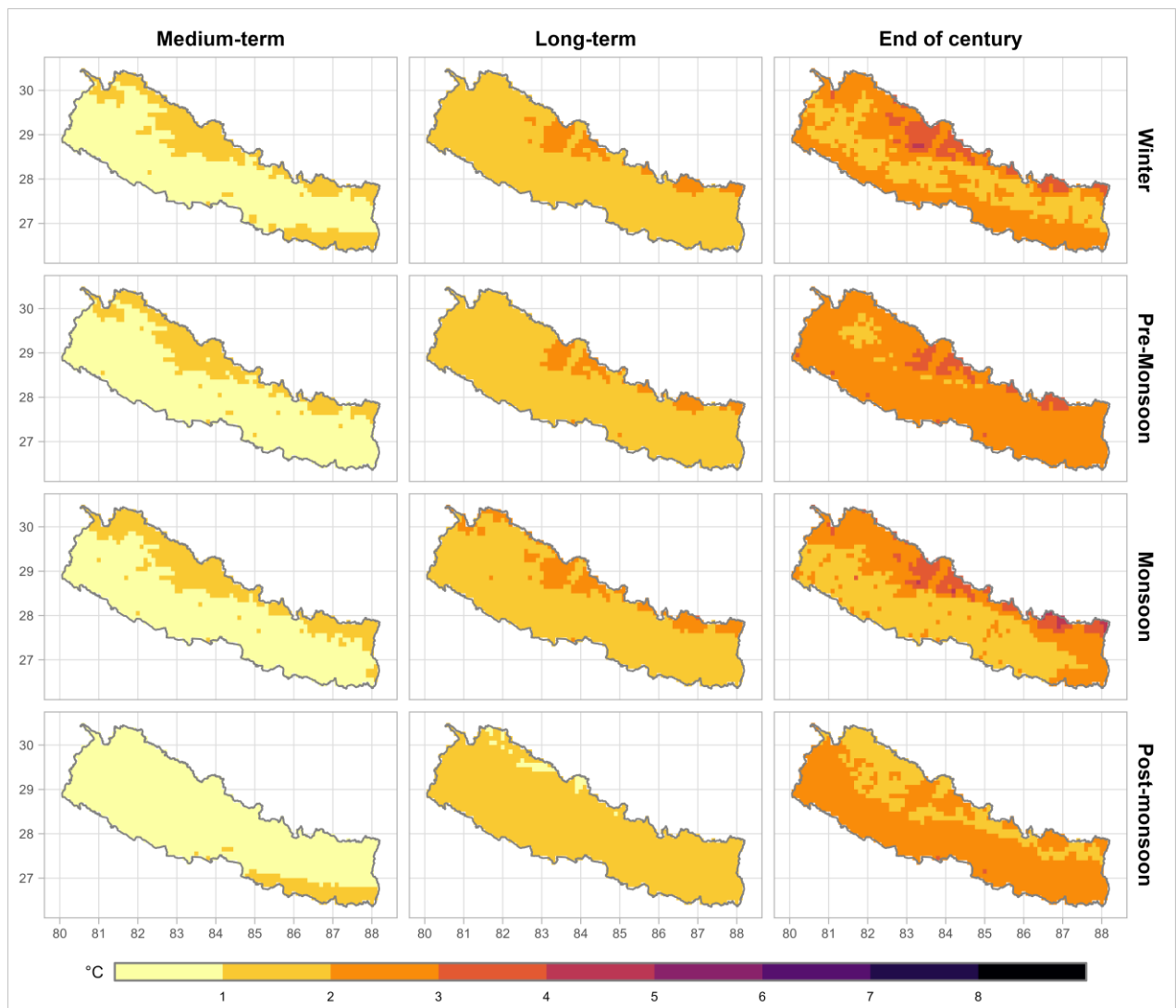
Figure 8.12: Spatiotemporal variation of projected change in seasonal minimum temperature (°C) during medium-term, long-term and end of century compared to the baseline period (1981–2010) for SSP2-4.5 scenario. Results are an ensemble average of selected four models.
