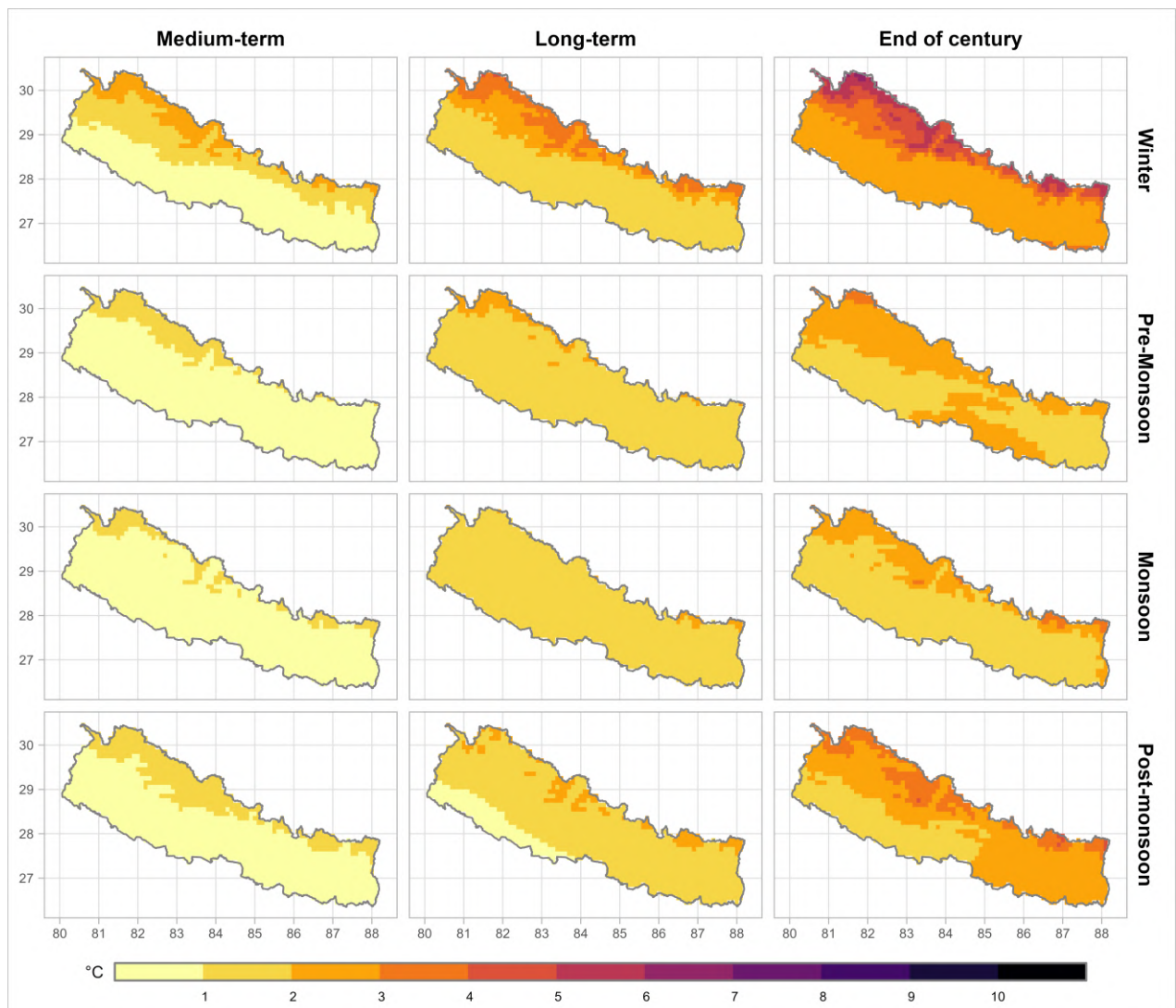
Figure 8.10: Spatiotemporal variation of projected change in seasonal maximum temperature (°C) during medium-term, long-term and end of century compared to the baseline period (1981–2010) for SSP2-4.5 scenario. Results are an ensemble average of selected four models.
