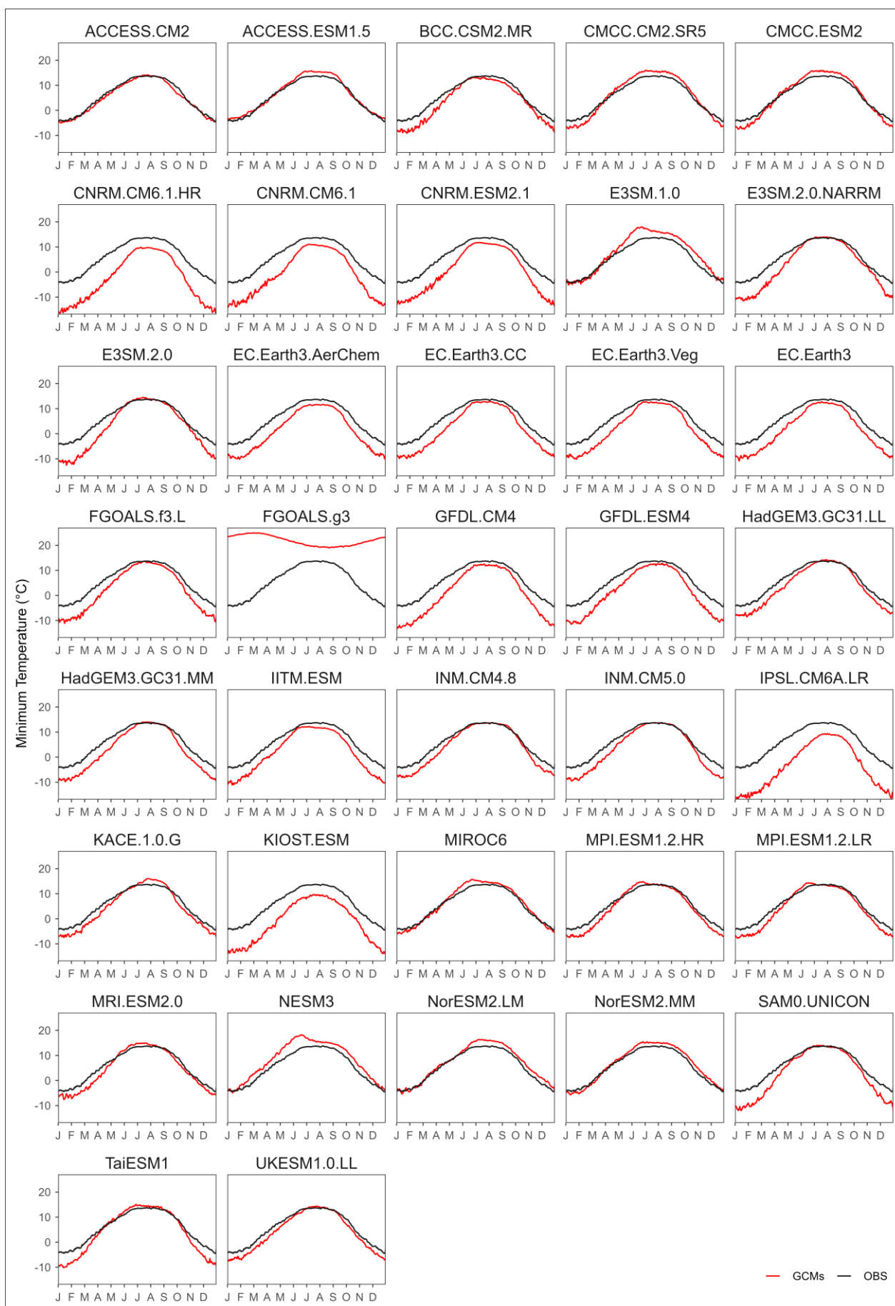
Figure 8: Comparison of daily minimum temperature climatology (mm) between observed and GCM data during the baseline period (1981–2010).
