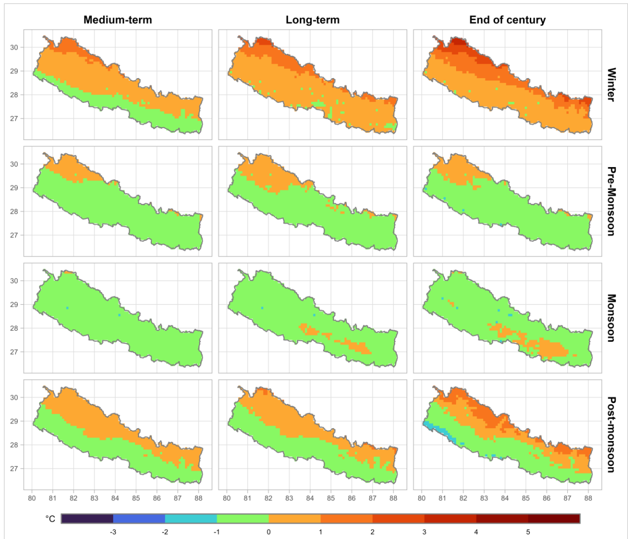
Figure 8.14: Spatiotemporal variation of projected change in seasonal diurnal temperature range (°C) during medium-term, long-term and end of century compared to the baseline period (1981–2010) for SSP2-4.5 scenario. Results are an ensemble average of selected four models
