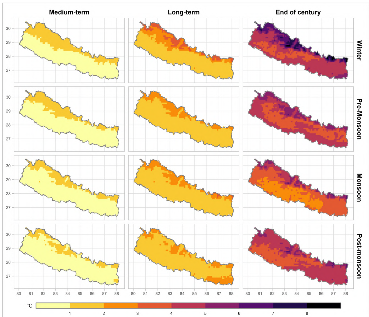
Figure 8.9: Spatiotemporal variation of projected change in seasonal mean temperature (°C) during medium-term, long-term and end of century compared to the baseline period (1981–2010) for SSP5-8.5 scenario. Results are an ensemble average of selected four models.
