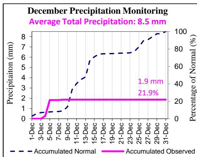
Figure 3: Cumulative average of daily normal and observed precipitation during December 2023.
