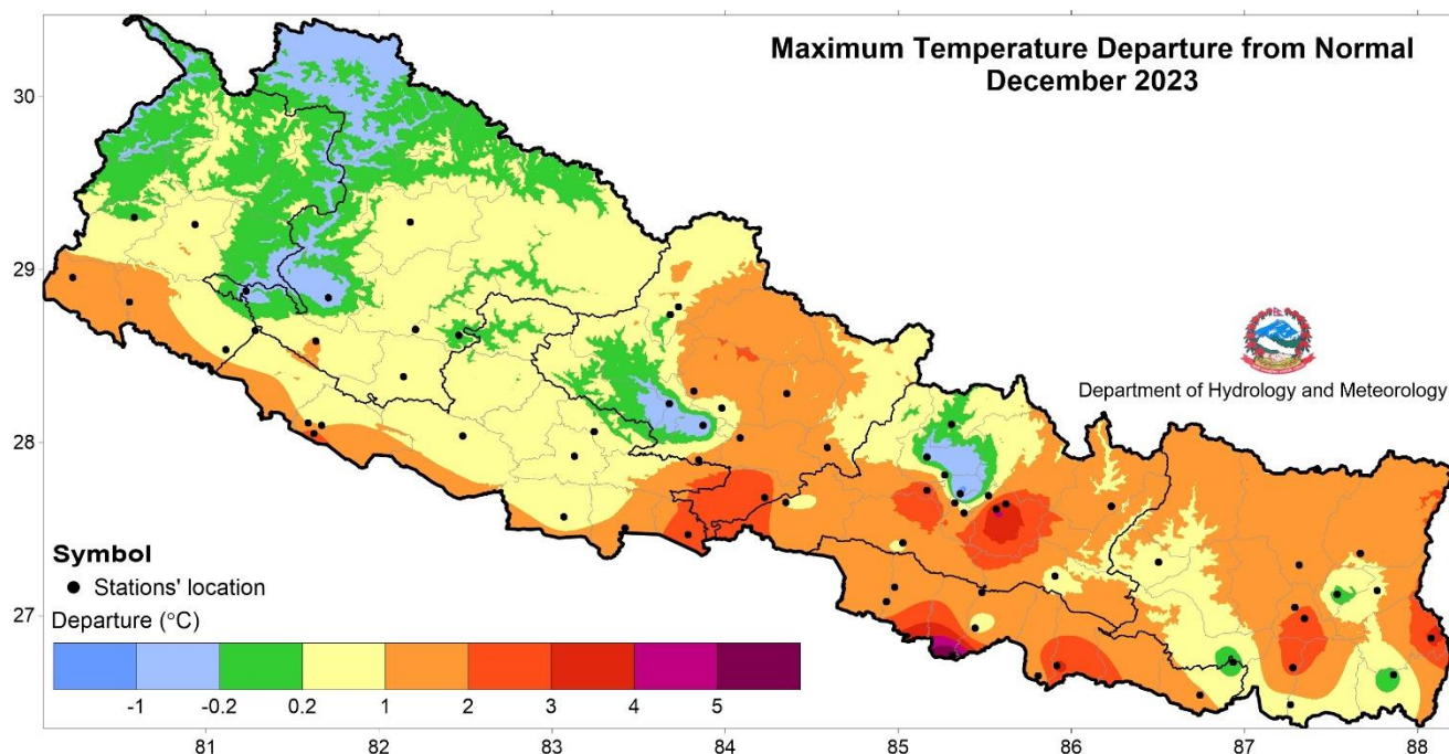
Figure 6: Departure from normal maximum temperature in December 2023.
