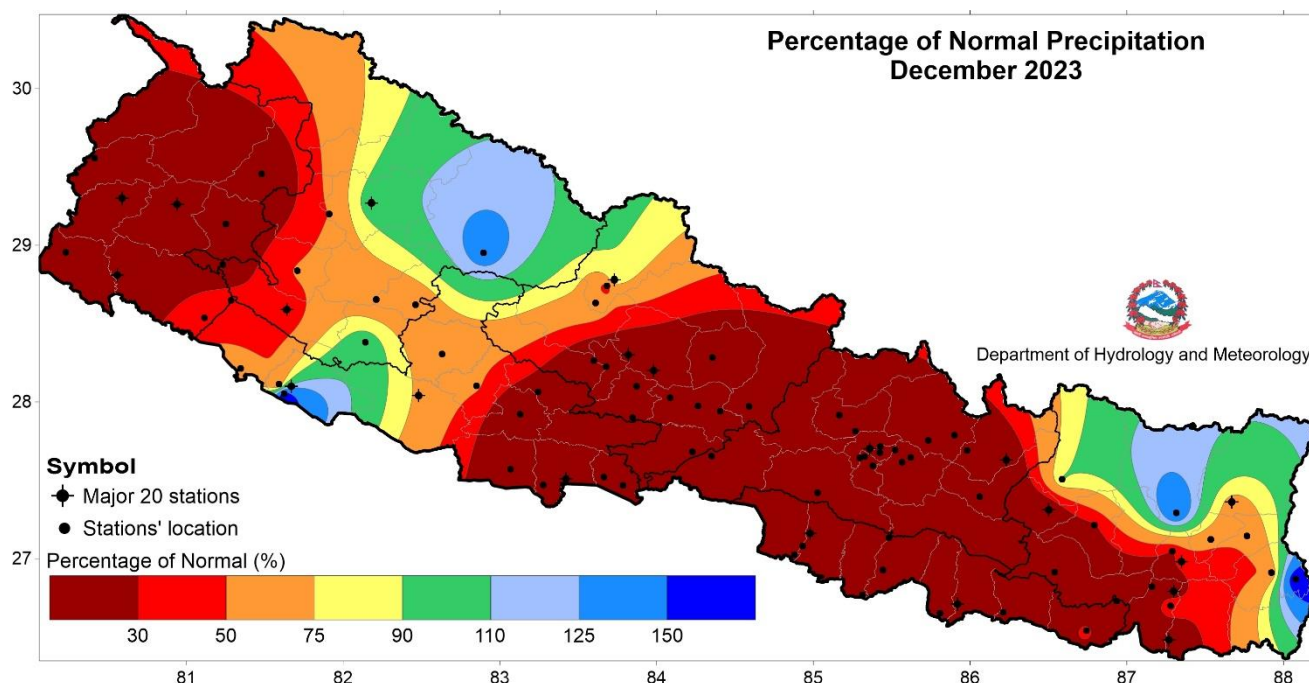
Figure 2: Percentage of normal precipitation in December 2023.
