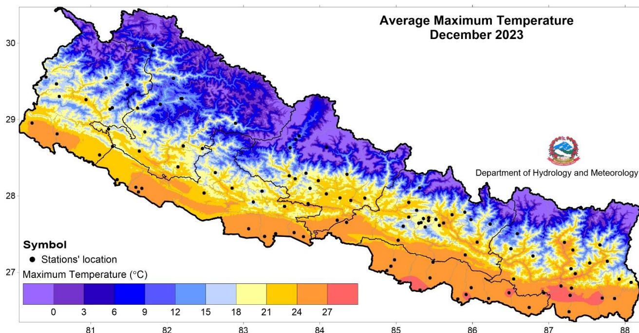
Figure 5: Maximum Temperature in December 2023.
