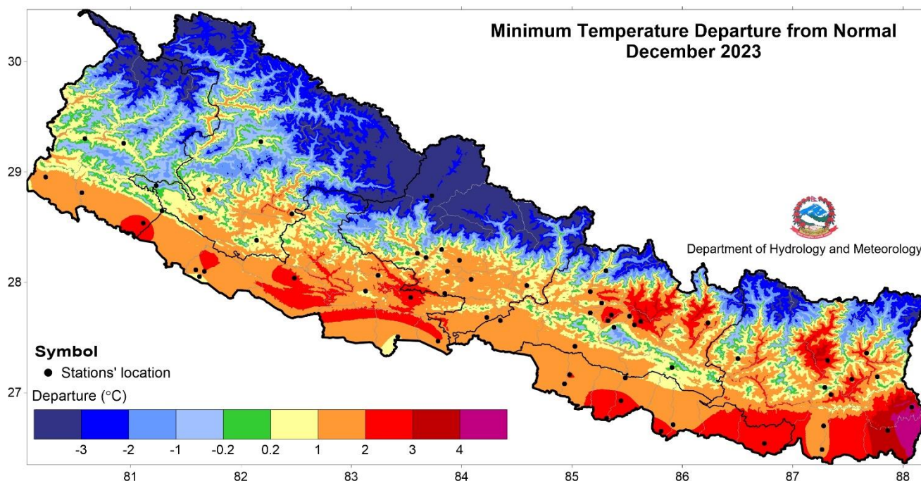
Figure 8: Departure from normal minimum temperature in December 2023.
