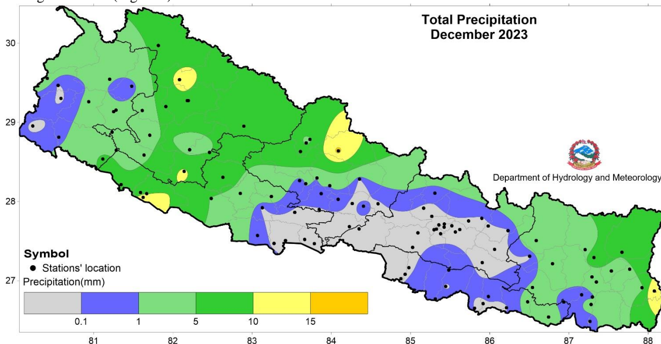
Figure 1: Total precipitation in December 2023.
