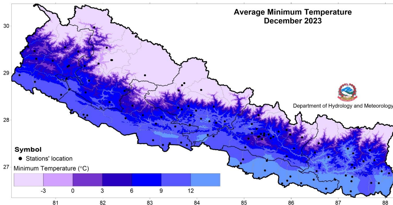
Figure 7: Minimum Temperature in December 2023.
