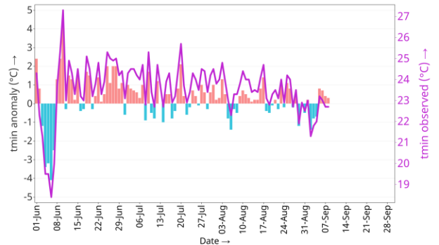
Minimum Temperature at Nepalgunj Airport
