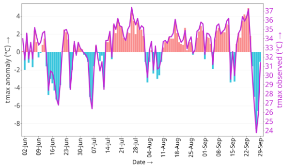
Maximum Temperature at Biratnagar Airport
