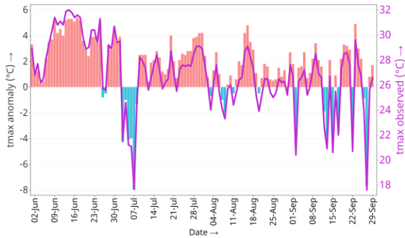
Maximum Temperature at Jumla
