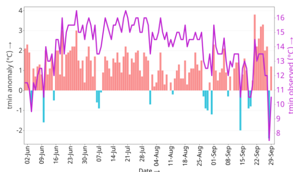
Minimum Temperature at Jomsom
