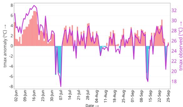
Maximum Temperature at Dadeldhura
