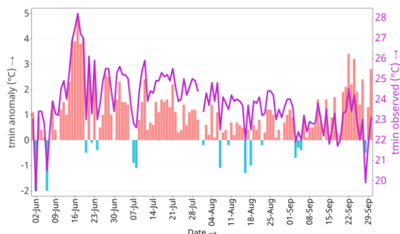
Minimum Temperature at Surkhet Airport (Birendranagar)
