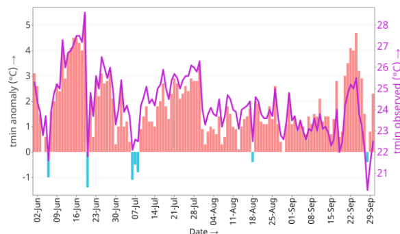
Minimum Temperature at Ghorai (Dang)
