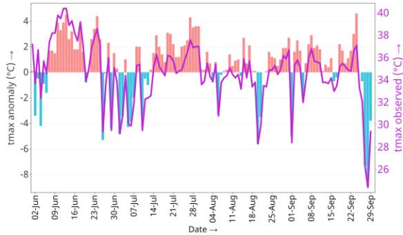
Maximum Temperature at Bhairahawa Airport
