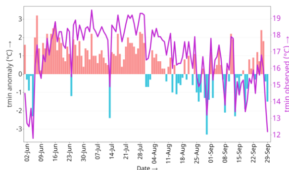
Minimum Temperature at Jiri
