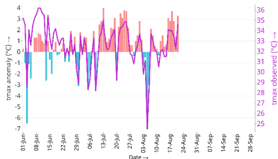
Maximum Temperature at Surkhet Airport (Birendranagar)
