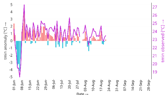
Minimum Temperature at Surkhet Airport (Birendranagar)
