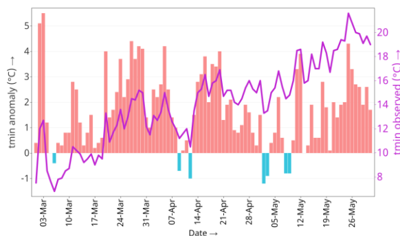
Minimum Temperature at Kathmandu Airport
