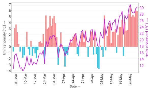
Minimum Temperature at Nepalgunj Airport
