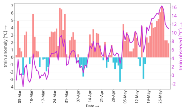
Minimum Temperature at Jumla
